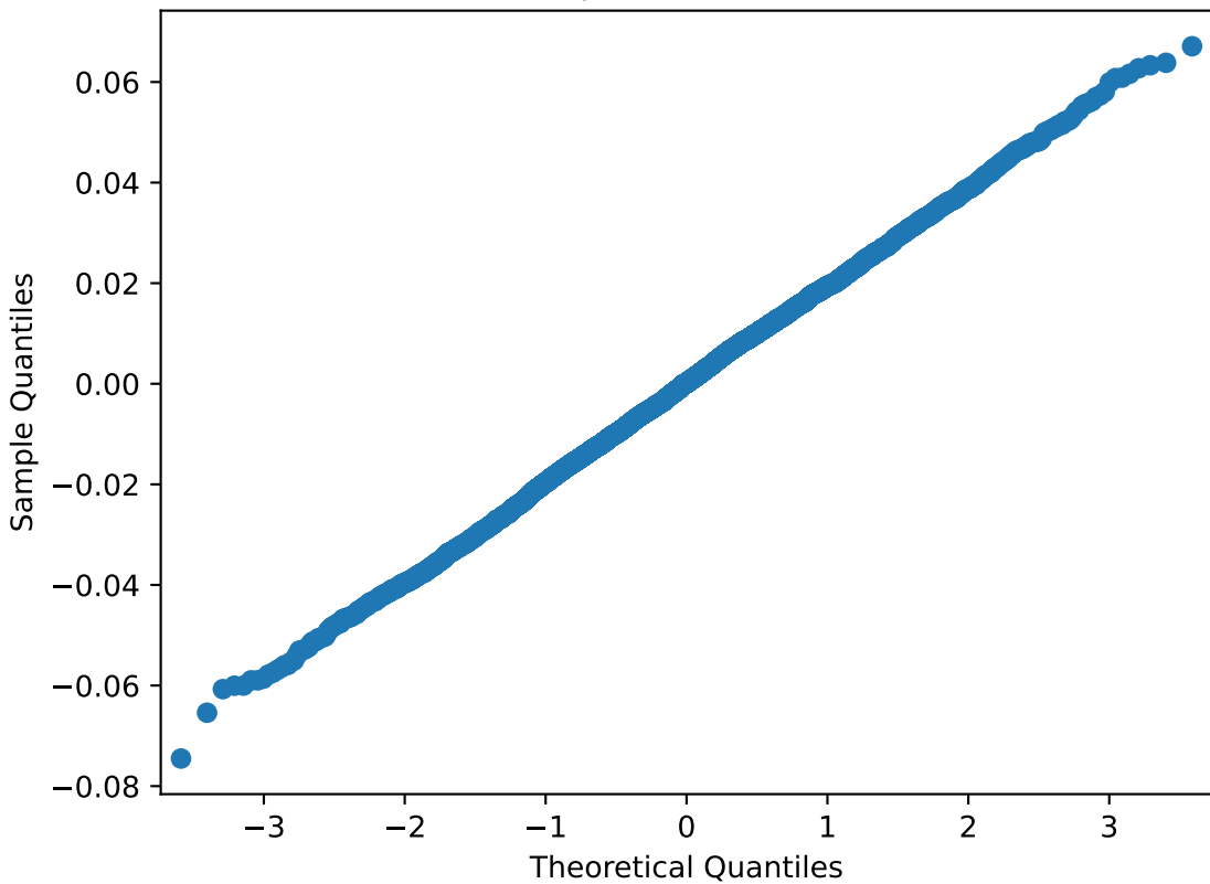
QQ-plot of residuals
